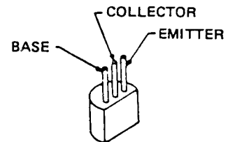
2SA733AP (Q7005-7008,7011 7012,7016,7018)
