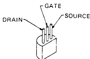
2SK125 (Q2004-2008,2011) 2SK104J (Q2020,2025)
