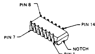
MC14066BCP (Q2026)
