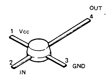
μPC1651G (Q2004-2006)
